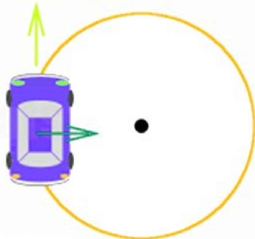
Centripetal force
