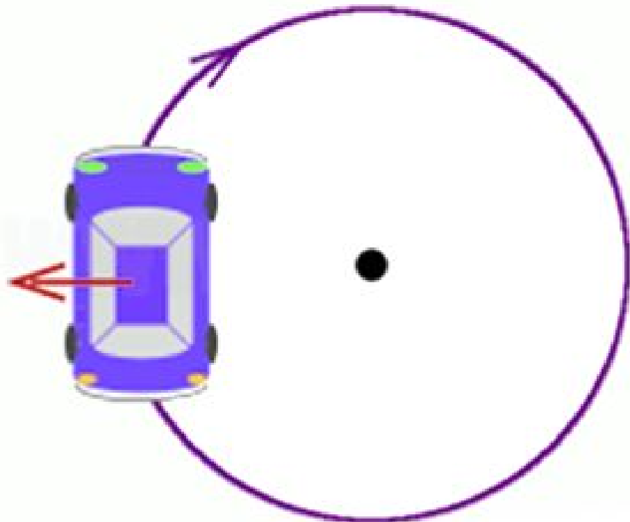
Centrifugal force
